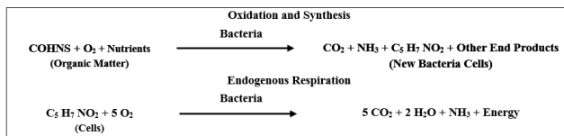
Fig. 5: Biological process happens in aeration zone
