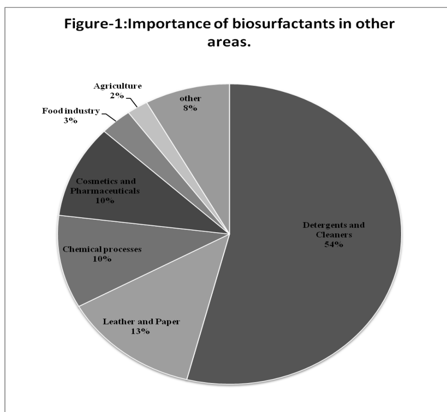
Fig. 1: Describes importance of biosurfactants in other areas (Rahman and Gakpe, 2008)
