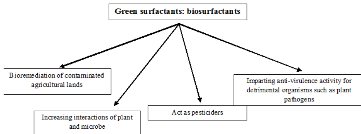
Fig. 2: Biosurfactant acceptance as green surfactants and their Importance in maintaining sustainability.
