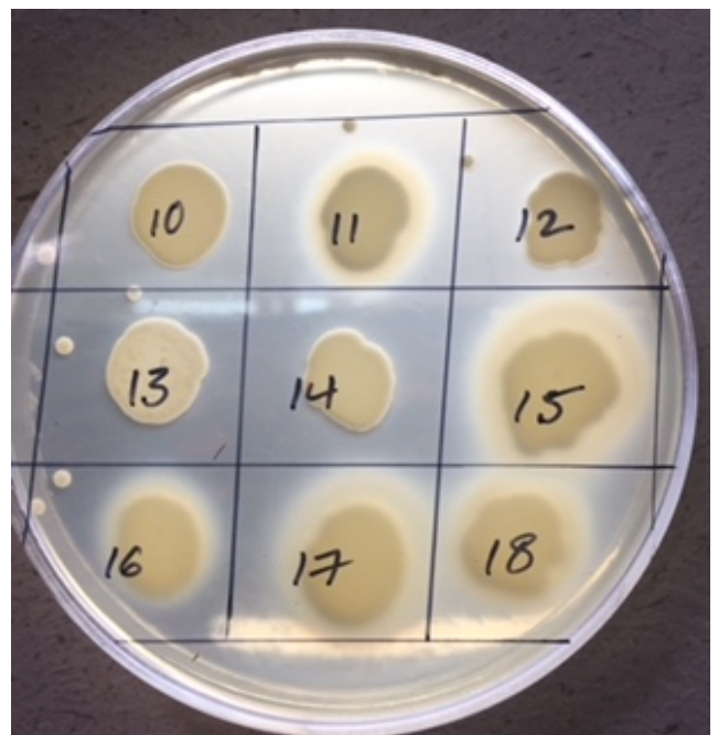
Fig. 5: Phospholipase production
