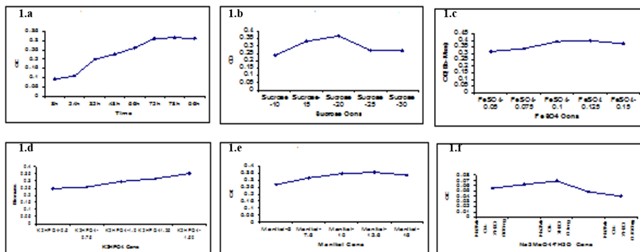
Fig. 1: Growth curve and association analysis; a: Explained the association between biomass (OD) or period of time; b: Correlation of sucrose cons and biomass (OD); c: Correlation of FeSO 4 cons and biomass (OD); d: Correlation of K 2 HPO 4 and biomass (OD); e: Correlation of manitol cons and biomass (OD); f: Correlation of Na 2 MoO 4 ·7H 2 O cons and biomass (OD)
